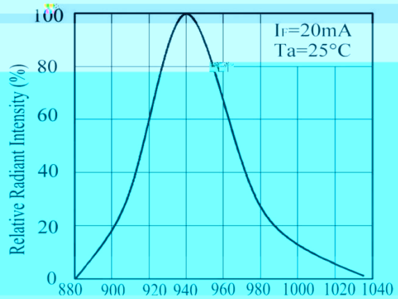
Fig.2 Spectral Distribution
